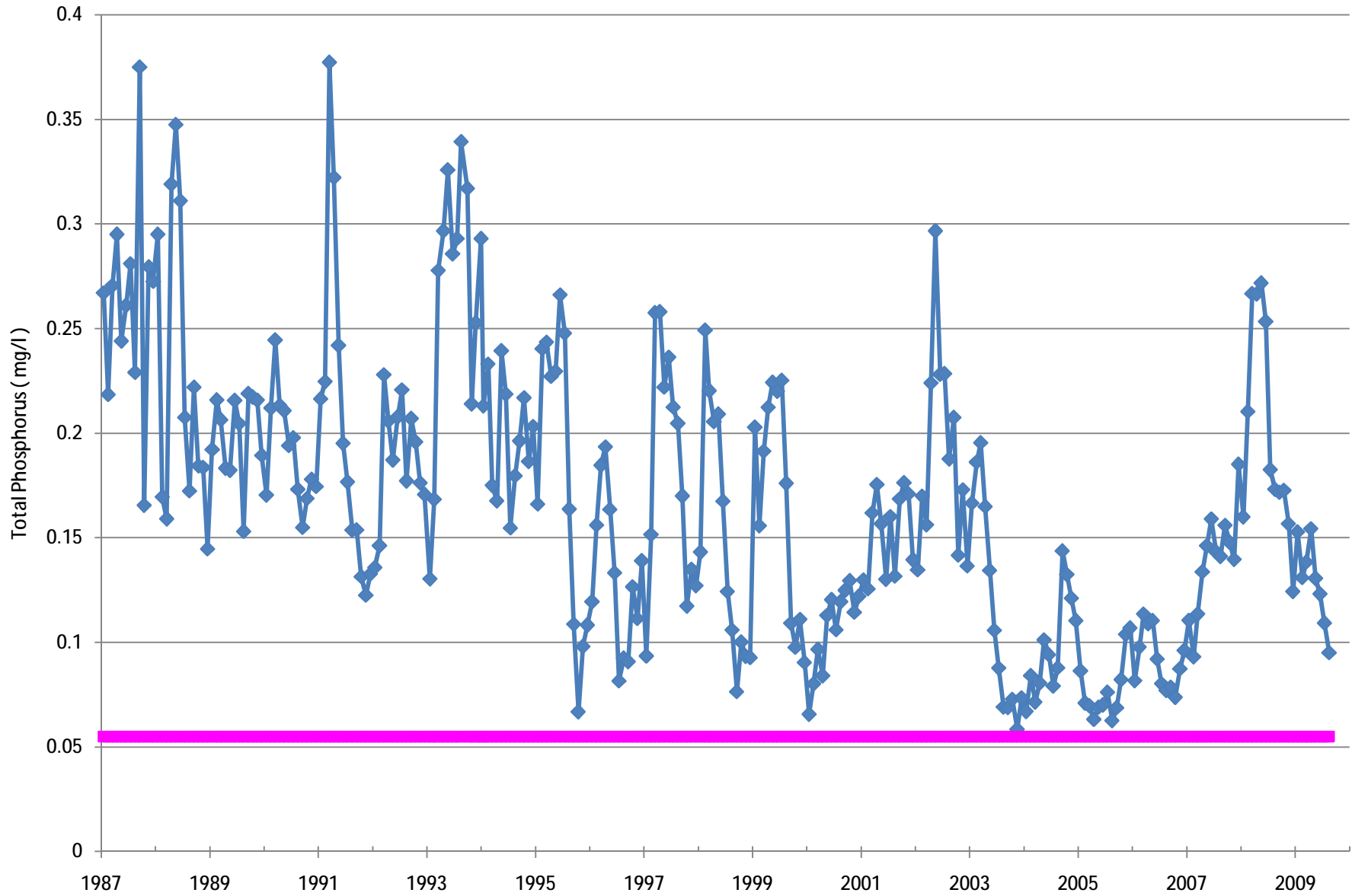
Lake Apopka Mean Monthly Total Phosphorus - 1987 through August 2009
